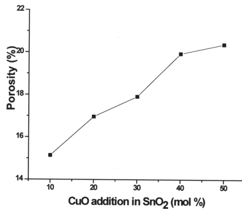
Fig. 6: Influence of CuO addition to porosity
